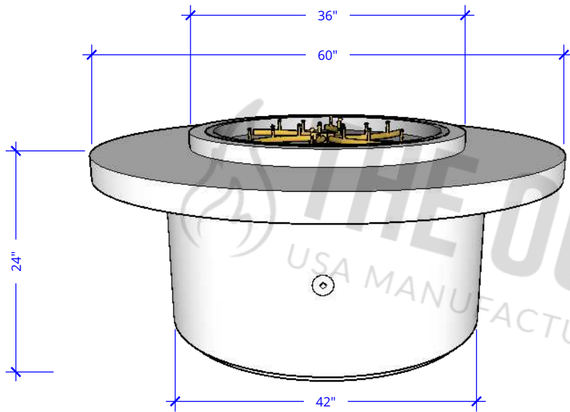
ISOMETRIC VIEW
