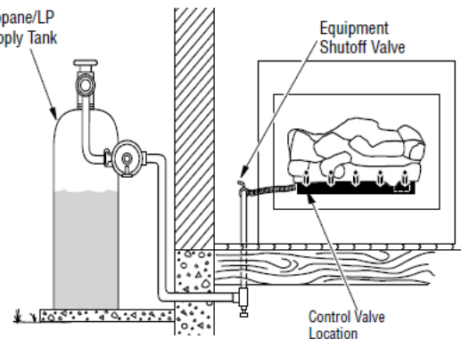
Figure C - External Regulator With Vent Pointing Down
