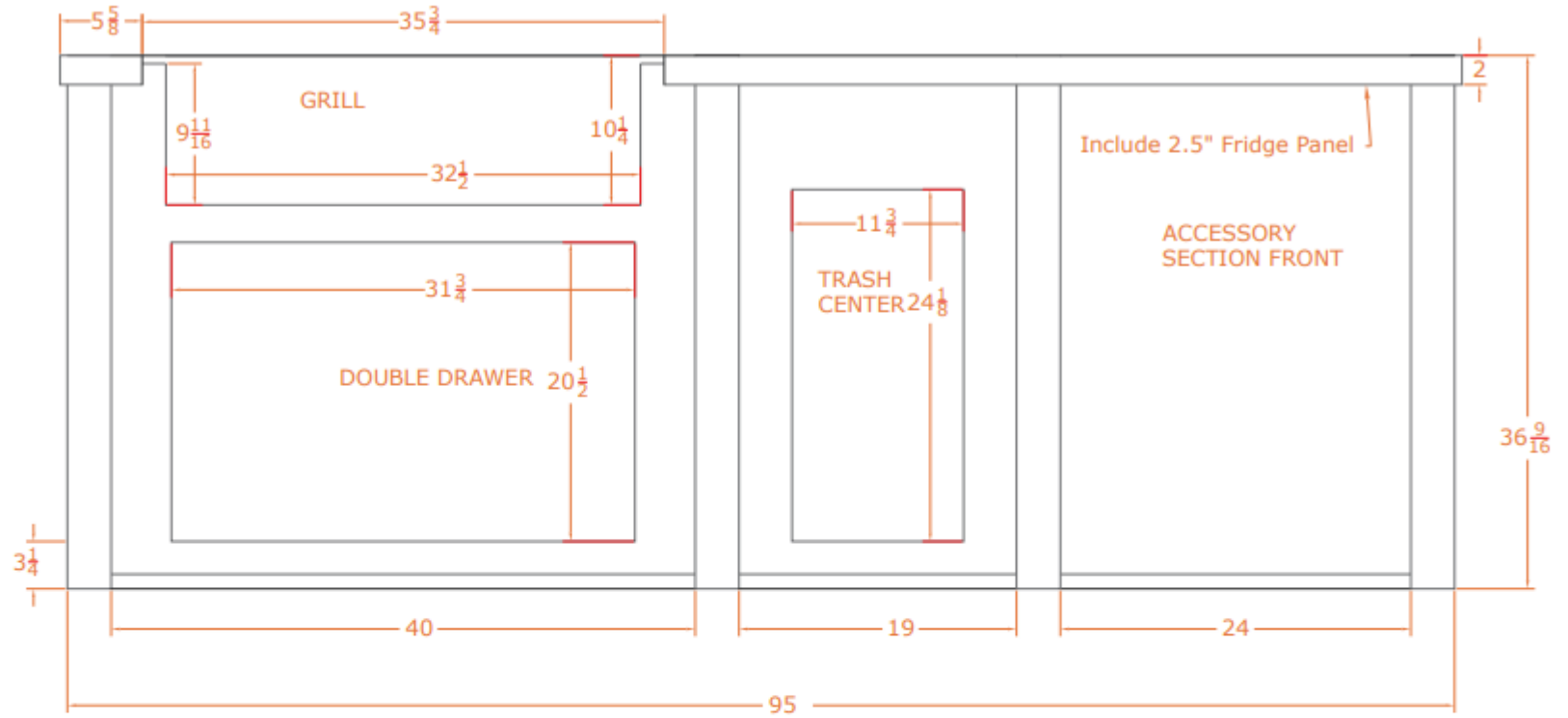
FRONT VIEW
